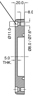
SECTION C-C
