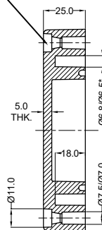
SECTION C-C
