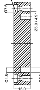
SECTION C-C
