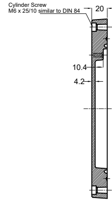
SECTION C-C
