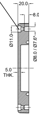
SECTION C-C
