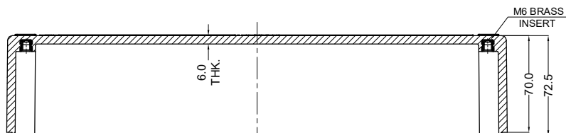
SECTION B-B
