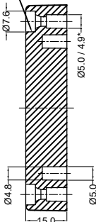
SECTION C-C
