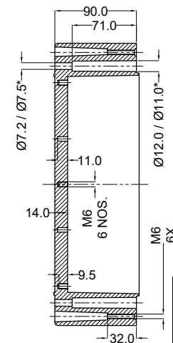
SECTION B-B
