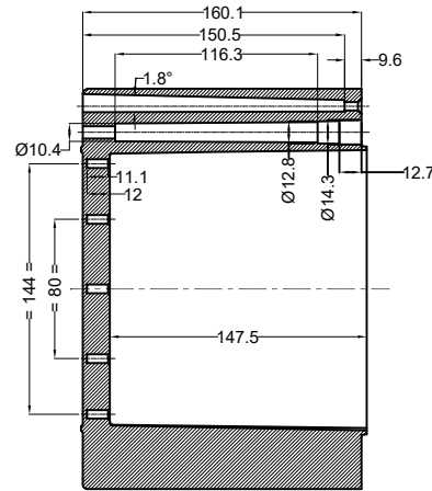
SECTION B-B
