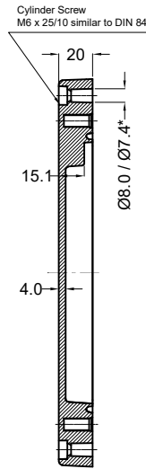
SECTION B-B
