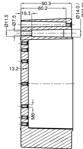
SECTION B-B
