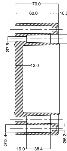
SECTION B-B
