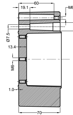
SECTION B-B
