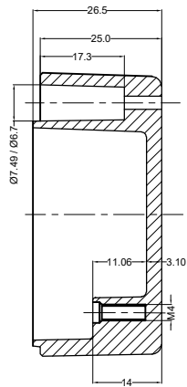
SECTION B-B
